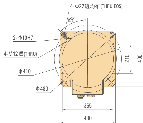
底座安装图 Base installation drawing
