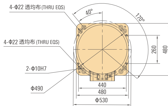
底座安装图 Base installation drawing
