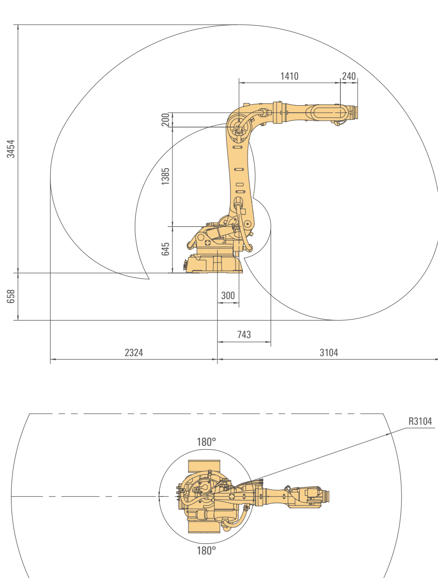
外形尺寸及运动范围 Outline dimension and Working range
